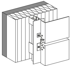
2 CASSETTE SCREWED for vertical façade structuring
