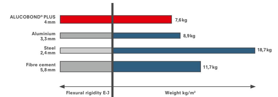
Comparison of thickness and weight with the same flexural rigidity
